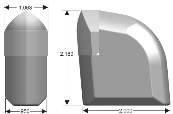
PART # 2180-1063
