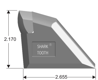
PART # SH300-N
