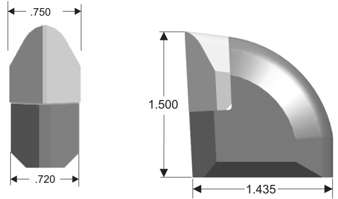
PART # 1500-47
