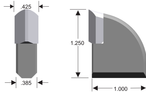
PART # 1250-38
