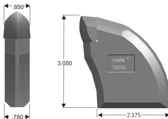
PART # SH300-875
