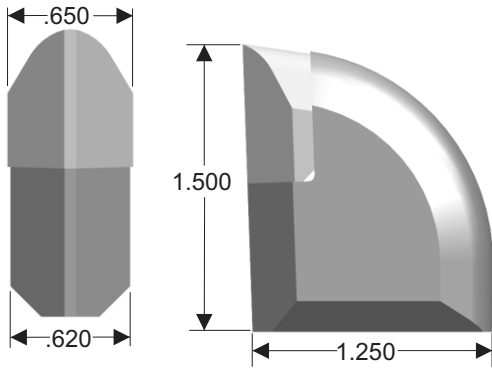
PART # 1500-650
