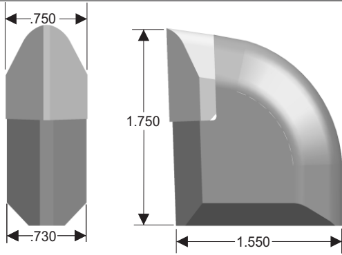
PART # 1750-47
