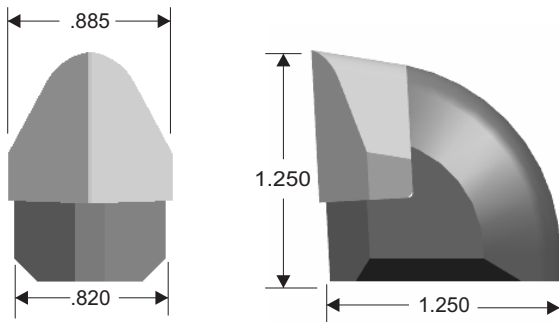
PART # 300-250
