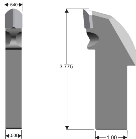
PART # 1654-LS
