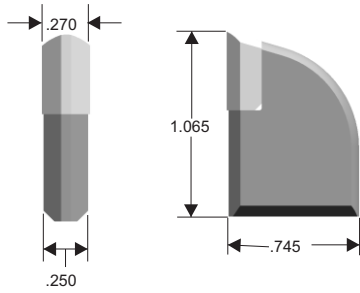
PART # 1065-250
