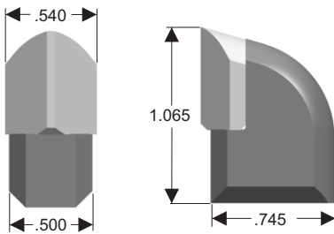
PART # 1065-50
