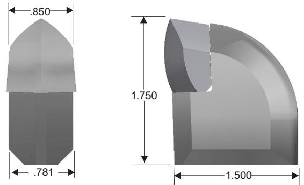
PART # 1750-04
