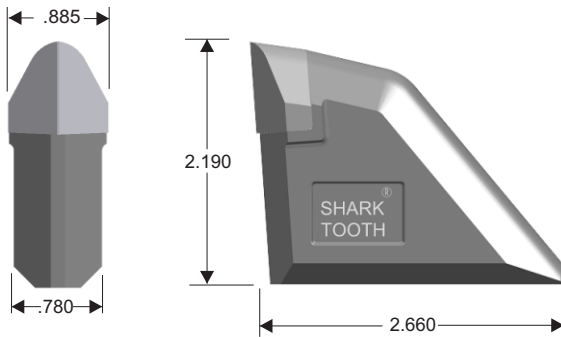
PART # SH300
