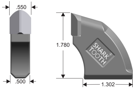
PART # SH1654
